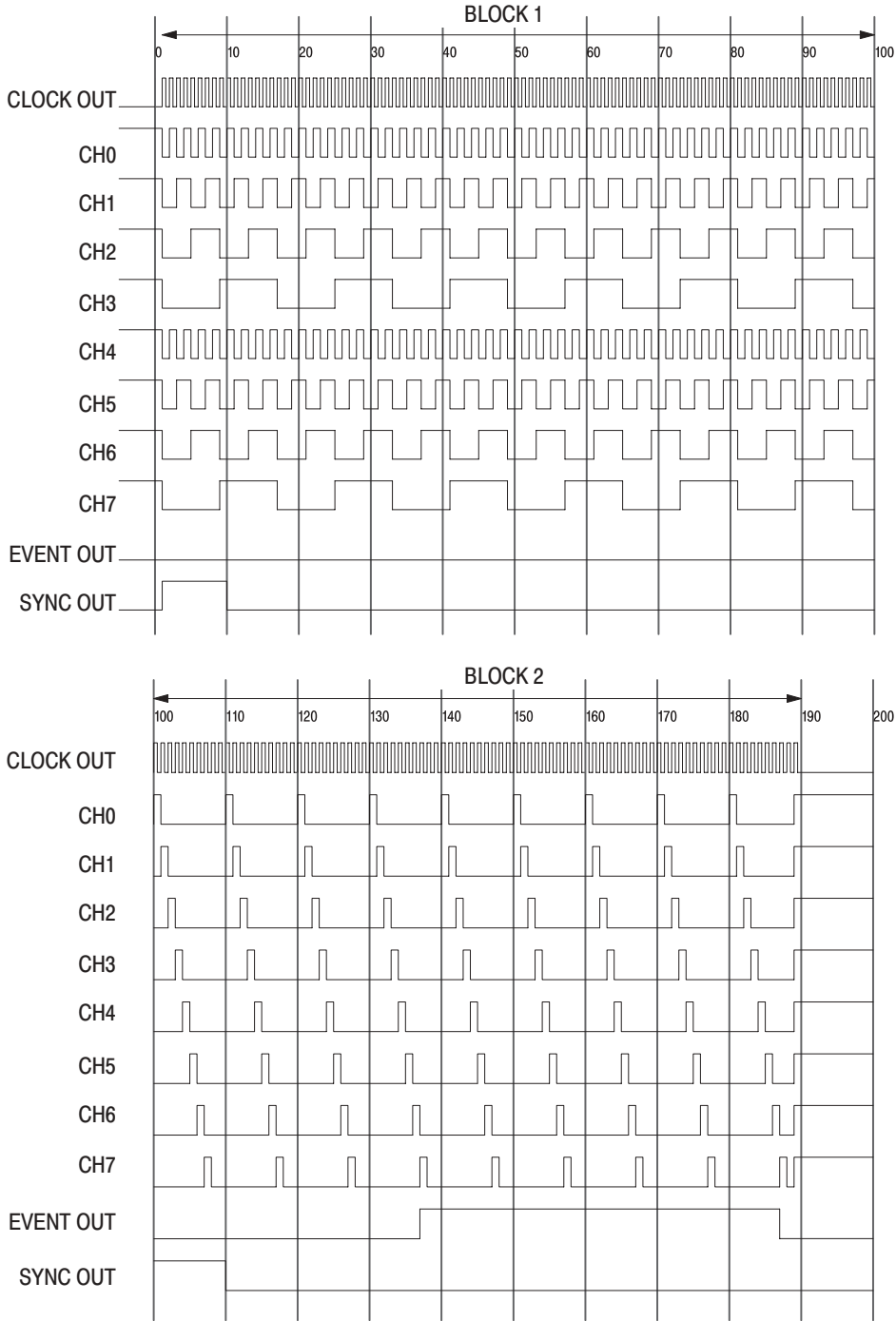
Figure B-8: Enhanced timing chart
