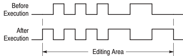
Figure 3-26: Invert data
