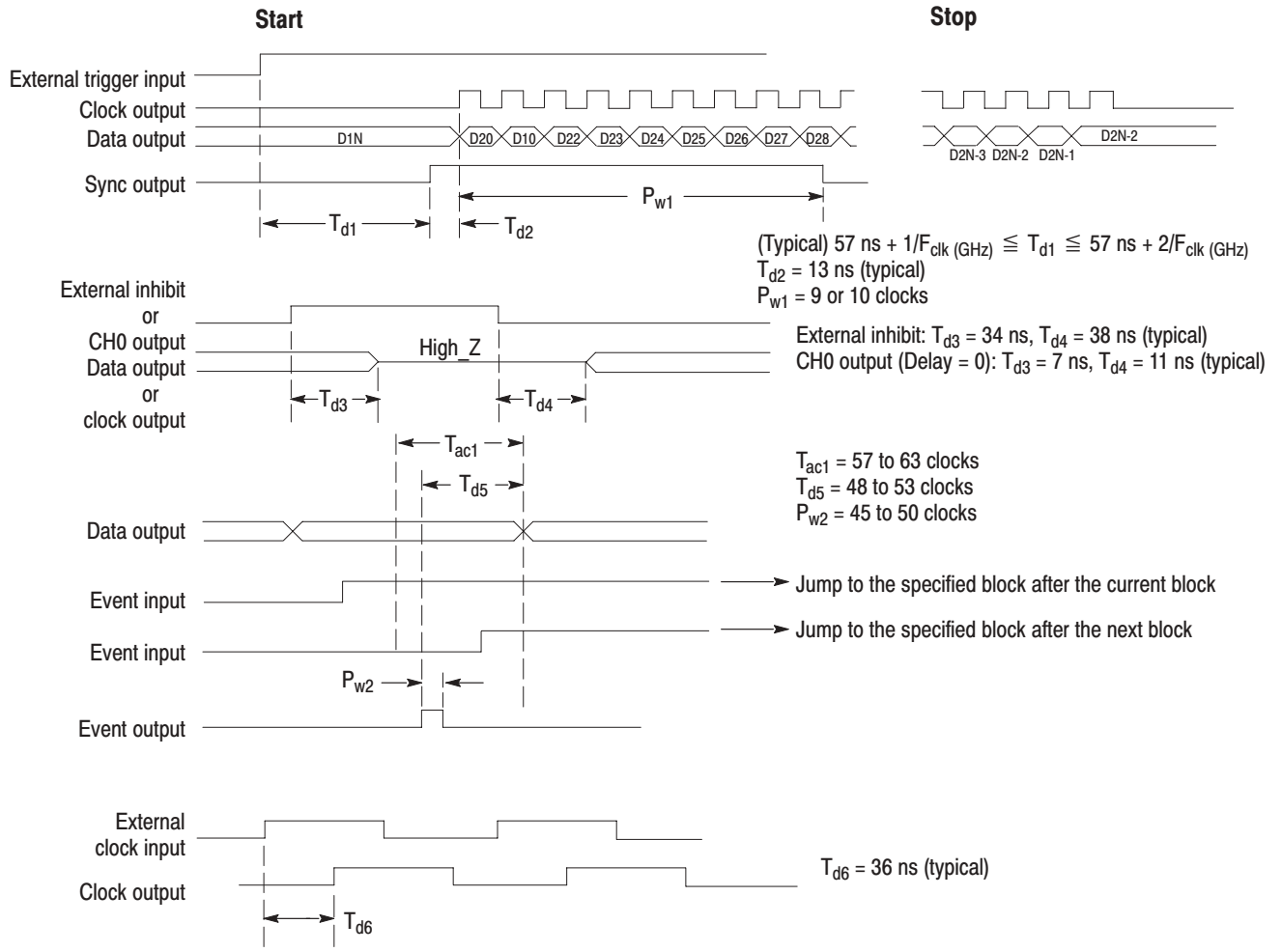
Figure A-2: Signal timing
