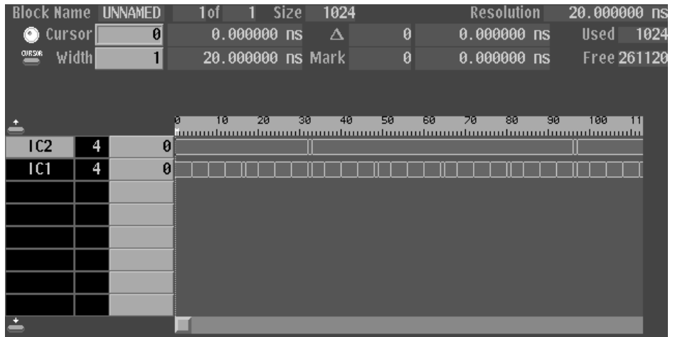
Figure 2-24: Group data
