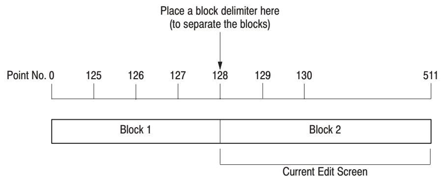
Figure 2-31: Block separation
